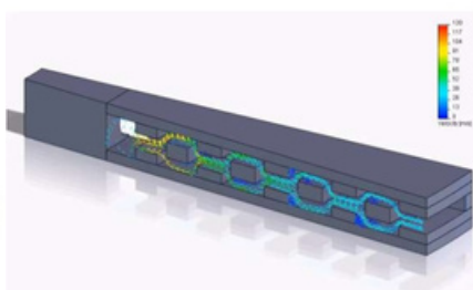
Inside Limiphon trim
